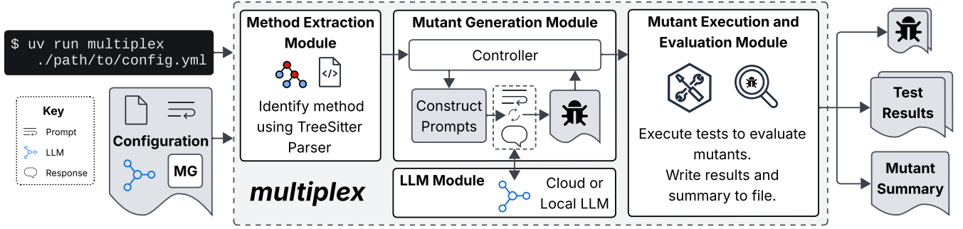
Figure 1: System overview of multiplex . Researchers can design and adapt each module to facilitate empirical studies.
