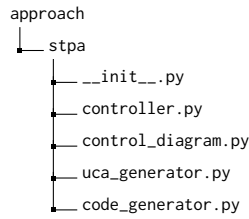
Figure 3: Mutant generation approach directory file structure example for m-STPA .
