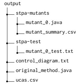
Figure 2: Output directory file structure example for m-STPA .
