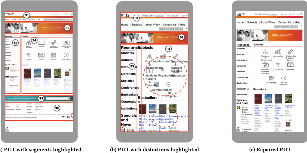
Figure 2: Example for demonstrating our approach. Thick red rectangles highlight segments identified by our technique, while dashed red ovals indicate distortions caused by undesirable adjustments to the page’s layout.
