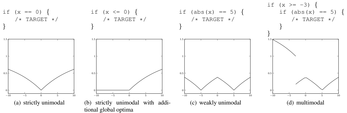
Figure 2: Examples of different fitness landscapes, including simple example code for a single variable x that generates these landscapes; \text{abs}(x) denotes the absolute value of x . To ease presentation, we used K = 0 in the branch distance and the base 1.001 of the normalisation function was changed to 1.1 for generating these plots. The function in (b) results from the strictly unimodal function (a) and adding global optima for x < 0 . In (d) values x < 3 lead to a high fitness value because of the worse approach level.
