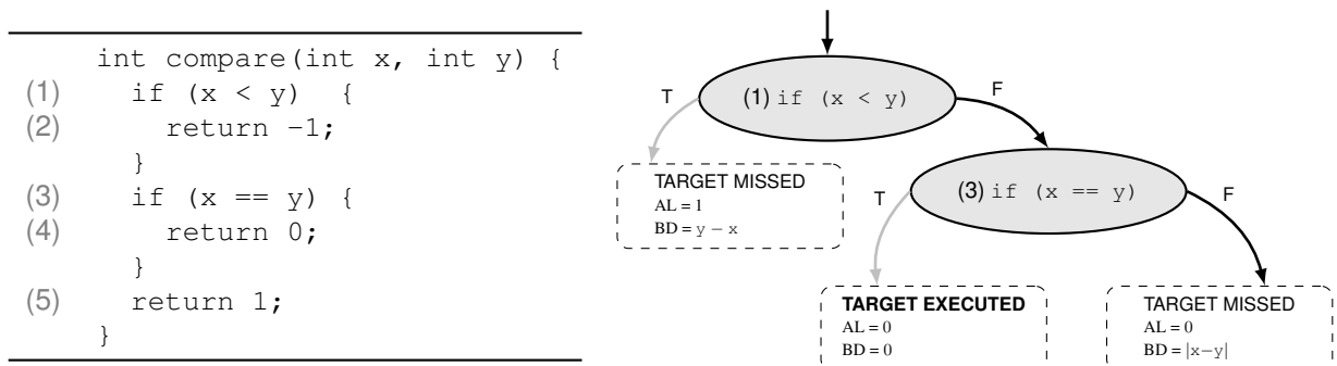
Figure 1: Example program for which branch-covering test inputs are required, and a partial control flow graph (CFG) showing fitness function computation (AL = approach level, BD = branch distance) for execution of the true branch from the second “ if ” statement of the program at CFG node (3) (corresponding control flow graph node numbers appear to the left of relevant code statements).
