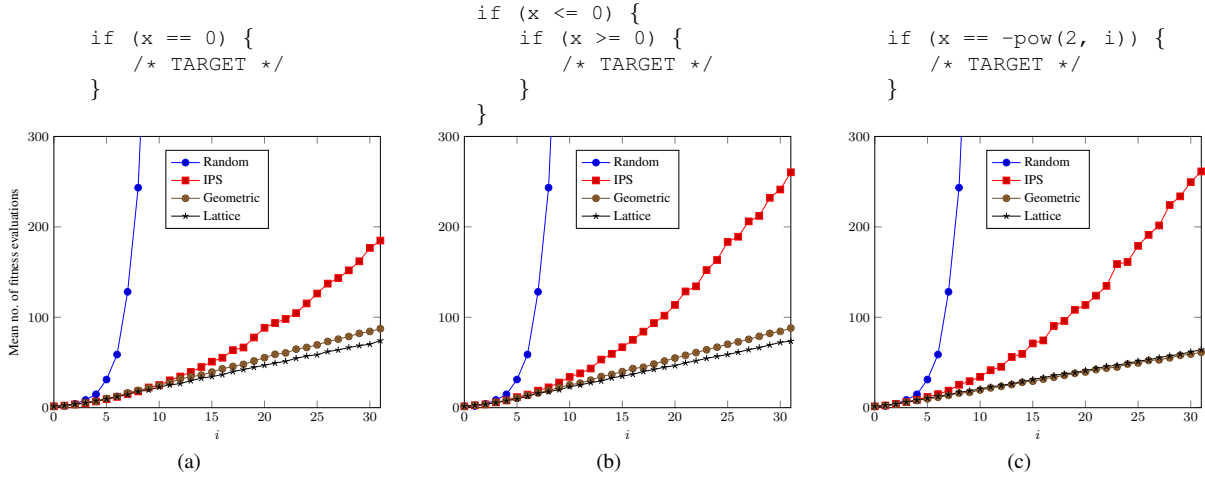
Figure 3: Comparisons of mean number of unique fitness evaluations for three strictly unimodal target branches with various local searches. The domain is chosen as \{-2^i, \dots, 2^i - 1\} for i \in \{0, \dots, 31\} . The first plot (a) corresponds to the function f(x) = |x| from Figure 2(a) and Theorem 3. The second branch (b) is similar, but all x > 0 have a worse fitness than all x \leq 0 . The third branch (c) shows a variant of (a) where the optimum is located at one end of the feasible domain.
