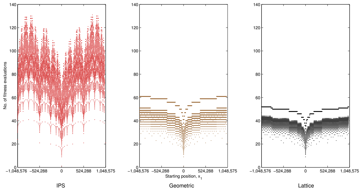
Figure 4: Number of unique fitness evaluations for optimizing f(x) = |x| with different local searches for each starting position x_1 \in [-2^{20}, 2^{20} - 1] . For the sake of clarity, the plots do not show all 2^{21} data points, but were downsampled to a selection of 25 000 data points for each search to give a good and accurate visual representation of all 2^{21} points, using the Largest-Triangle-Three-Buckets algorithm [27].
